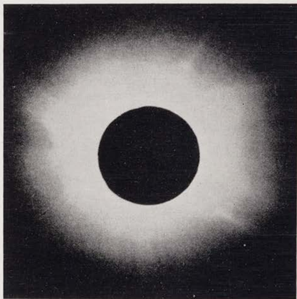
FIGURE 3—SHOWING CORONA MAXIMUM SUNSPOT SHAPE
